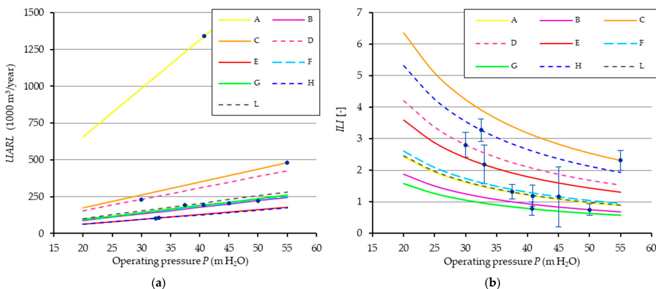
Figure 1. The influence of variable values of average operating pressures in the water supply networks on values of: (a) unavoidable annual real loss (UARL) and (b) infrastructure leakage index (ILI) calculated on the basis of actual values of CARL. Plotted data represented by points show actual relationships between P and UARL and between P and ILI (with error bars).
